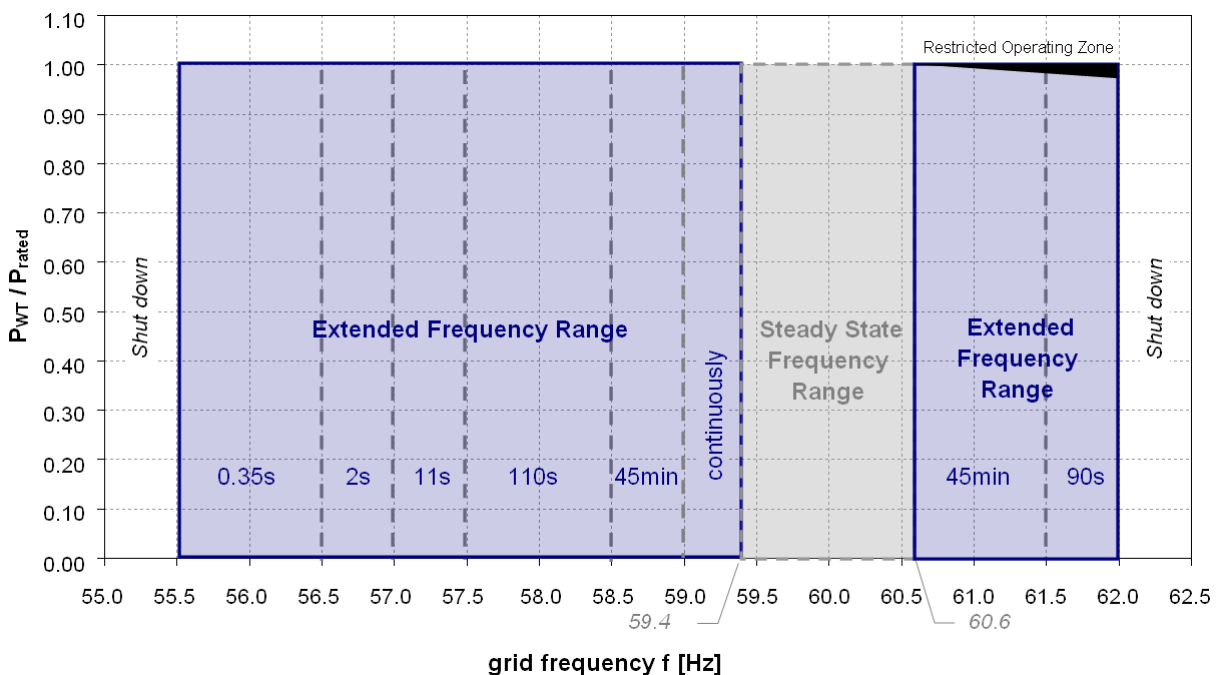
Figure 2: Extended Frequency Range of REpower MM92 CCV
